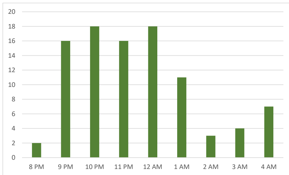
FIGURE 4. AVERAGE BAT ACTIVITY PATTERNS THROUGHOUT THE NIGHT.
