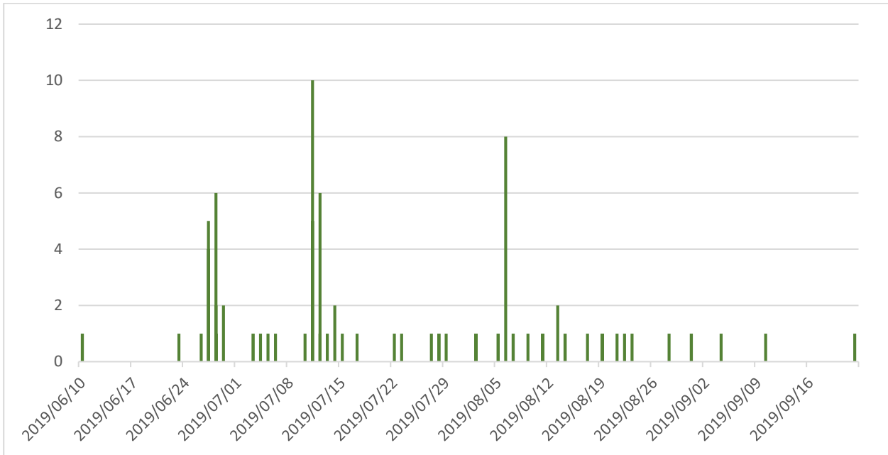
FIGURE 3. BAT ACTIVITY LEVEL OVER THE SEASON FOR ALL SPECIES.
