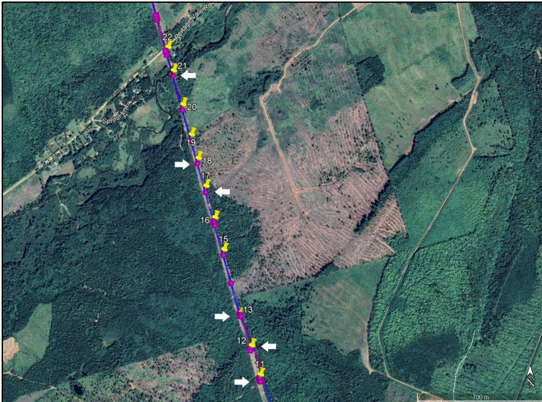
Figure 14: Phase 1 transmission line structure locations. White arrows point to areas monitored.
